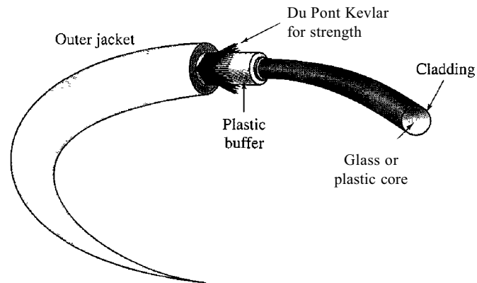
Figure 7.14 Fiber construction
